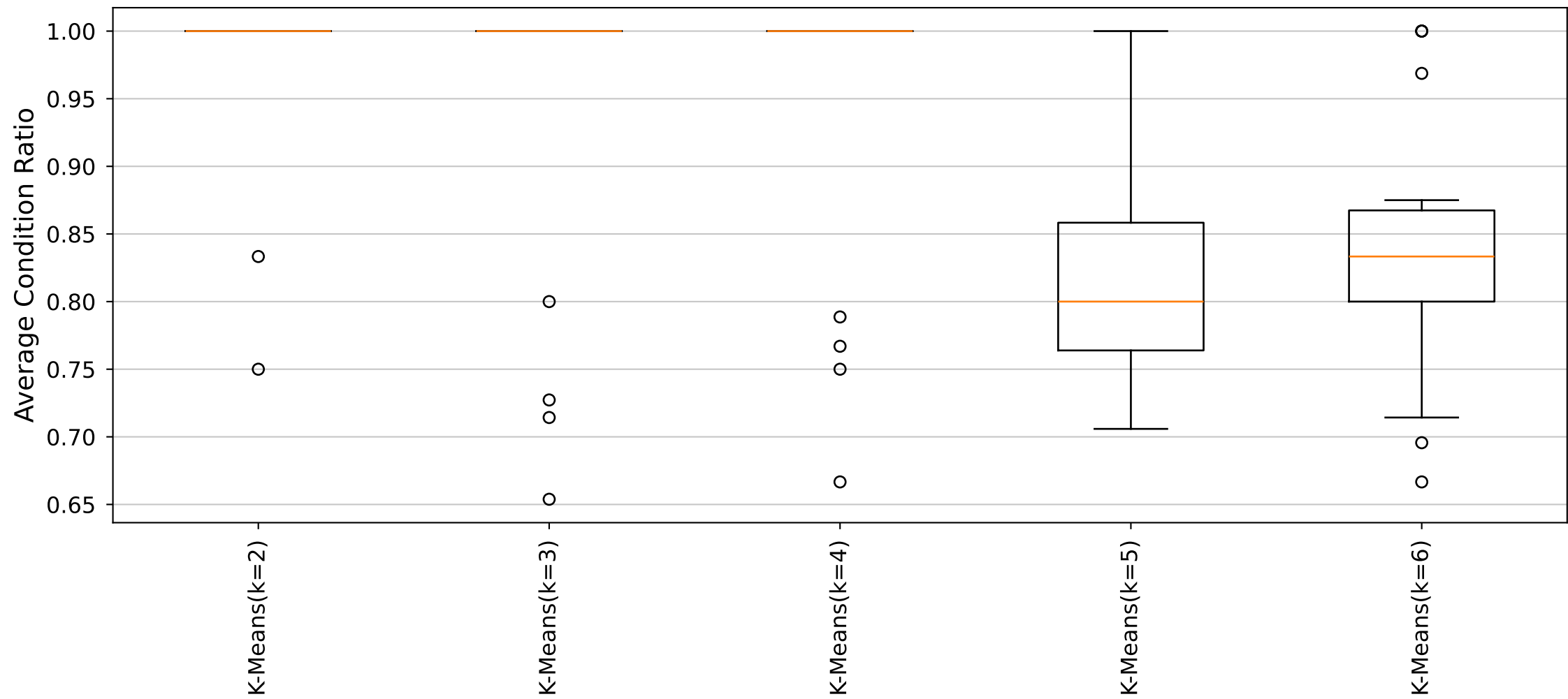
YARA Rules Average Condition Ratio Distribution (Cluster22_Size6 dataset)
